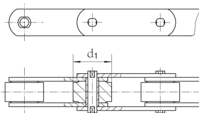
带P大滚子型 With P large roller type
