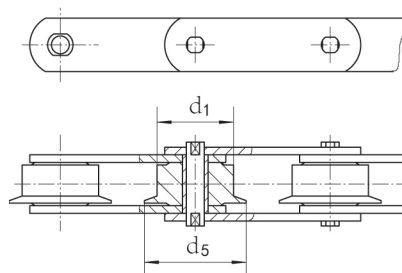
带F边滚子型 With F flanged roller type
