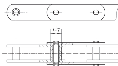
带F边滚子型 With F flanged roller type
