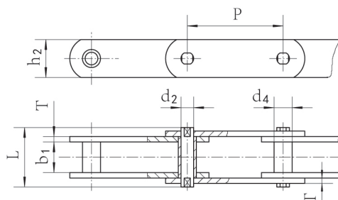
带P大滚子型 With P large roller type
