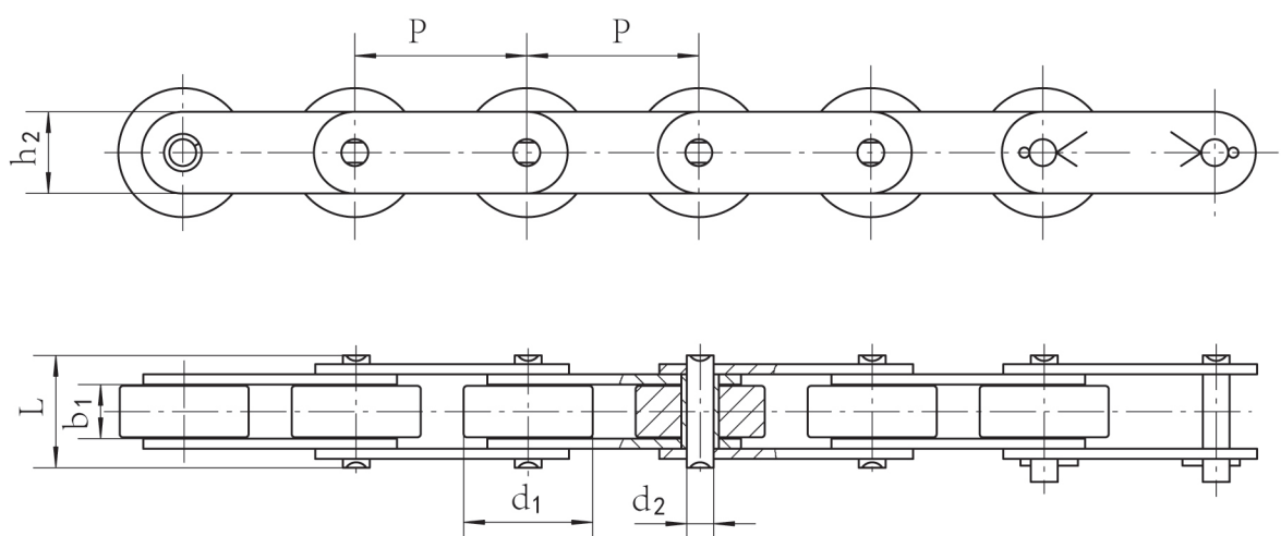
Oversize Roller Type
